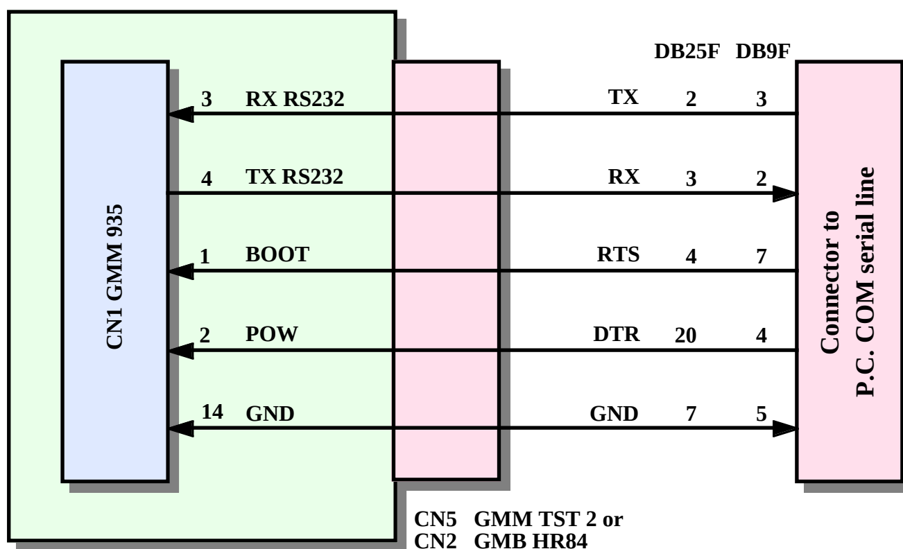
FIGURE 17: RS 232 SERIAL CONNECTION BETWEEN A GMM 935 AND A PC
