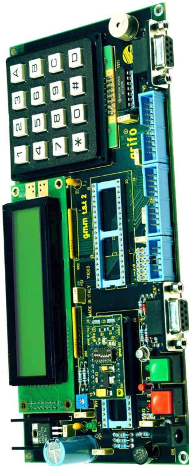
FIGURE 15: GMM TST2 + GMM 935 PHOTO
