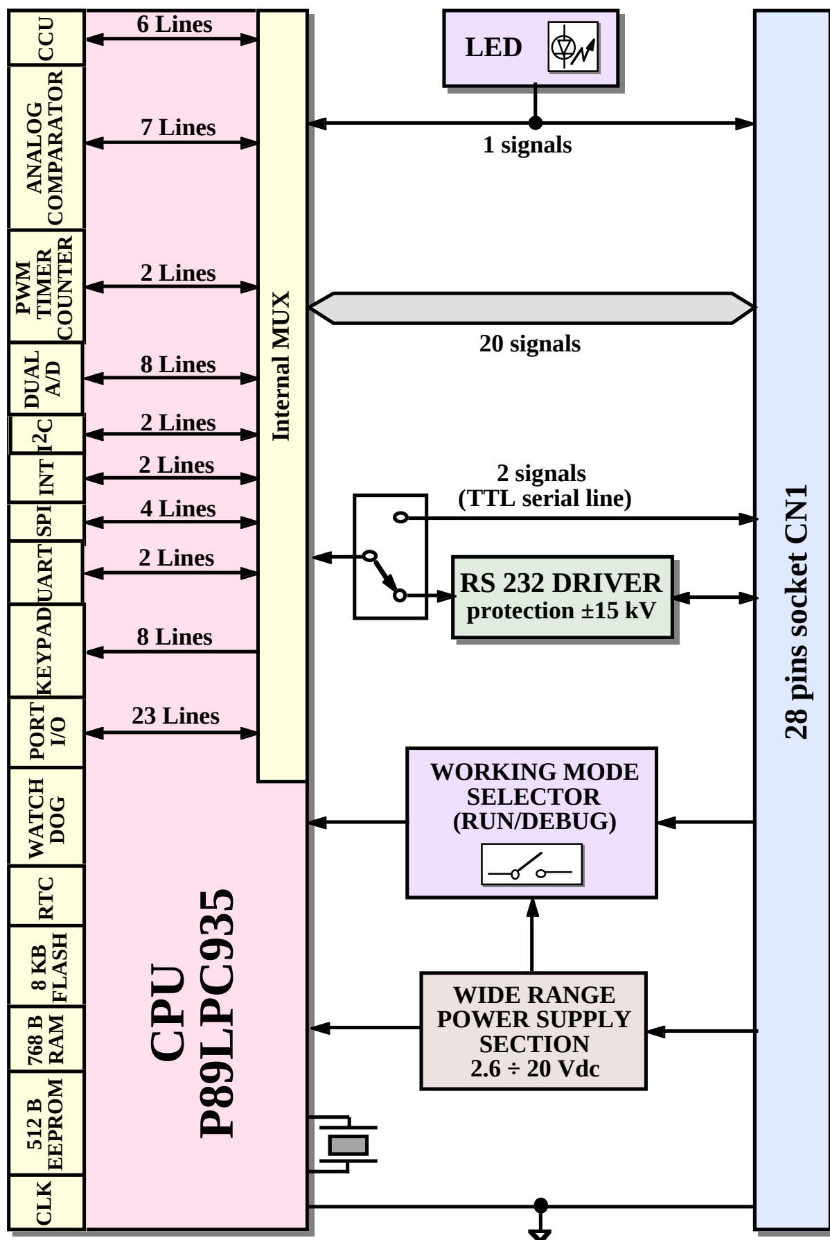
FIGURE 2: BLOCKS DIAGRAM
