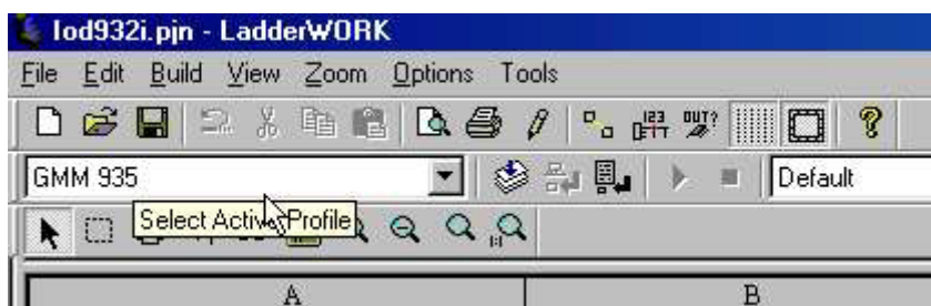
FIGURE 30: COMPILER CONFIGURATION FOR LADDER WORK
